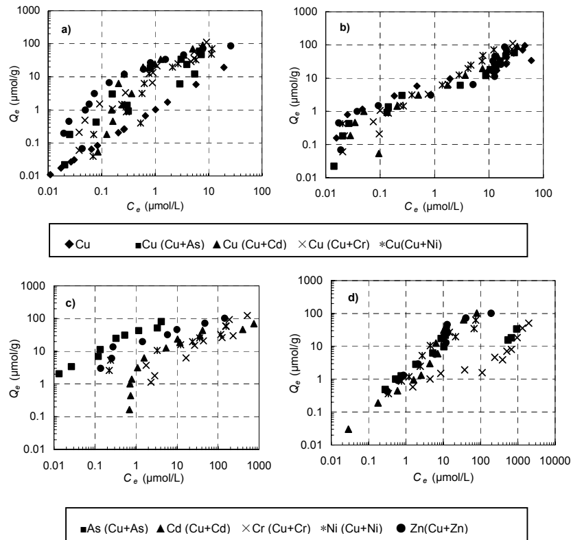
Fig. 1 Cu removed from water by a) alumina, b) GAC, and As, Cd, Cr, Ni and Zn in binary system removed from water by c) alumina, d) GAC; using sorbent dosage of 20 g/L, ionic strength ( I ) = 0.01M NaCl, start pH= 6.5±0.2
